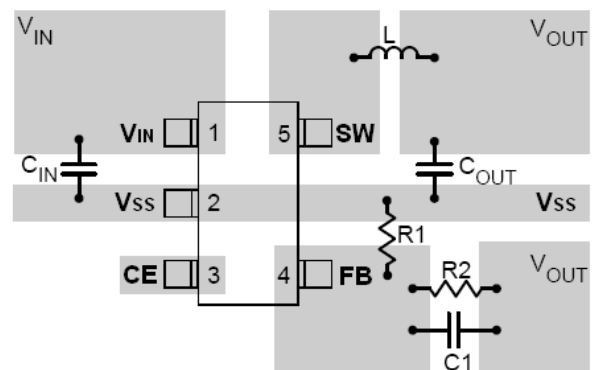
Figure2(b) LR8509AM Suggested Layout
