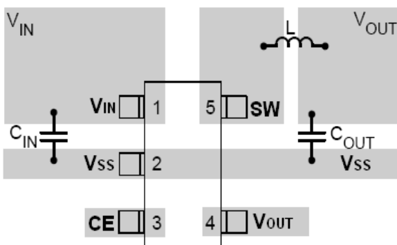
Figure2(a) LR8509A18M Suggested Layout
