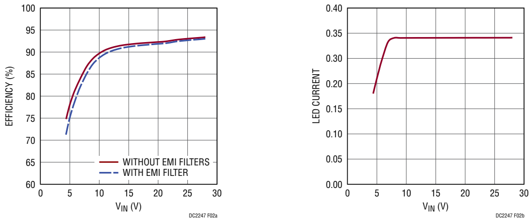
Figure 2. DC2247A Efficiency and LED Current Versus Input Voltage for 34V 330mA LED Load. Efficiency Remains High Through the Range Due to Synchronous Switching. At Low V IN , I LED Can Be Reduced Due to Peak Switch Current Limit
