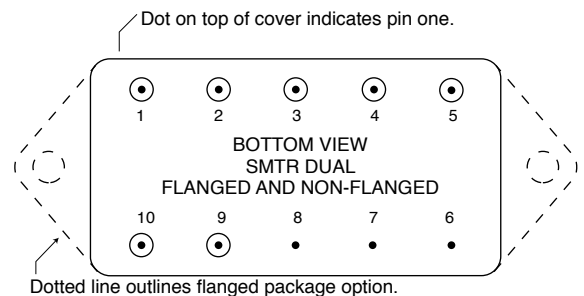
FIGURE 4: PIN OUT SMTR DUAL OUTPUT MODELS
