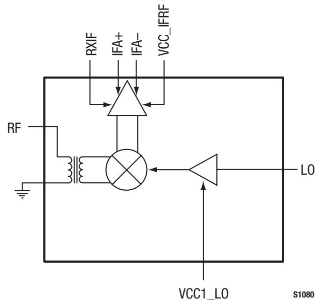
Figure 1. SKY73070 Block Diagram
