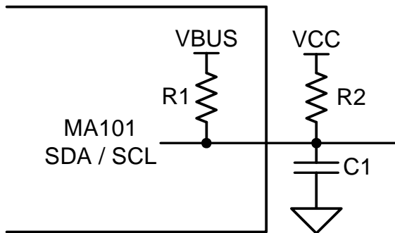
Figure 5-3 : Circuit diagram
