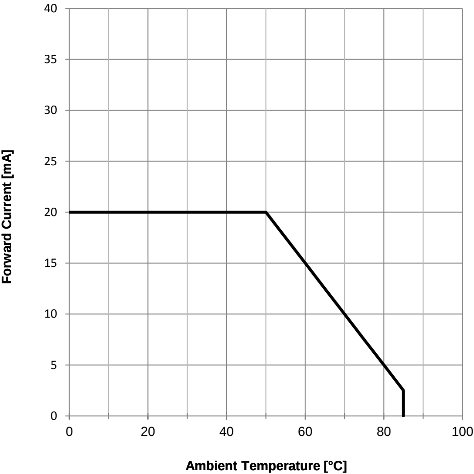
Derating Curve:
