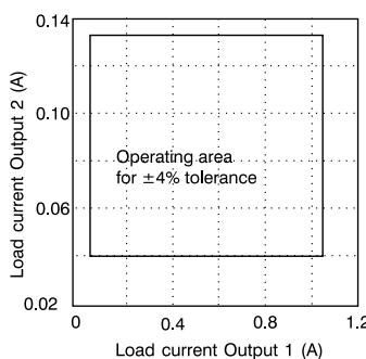
Cross regulation output 2 (-12V)
