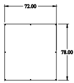
INNER PANEL
