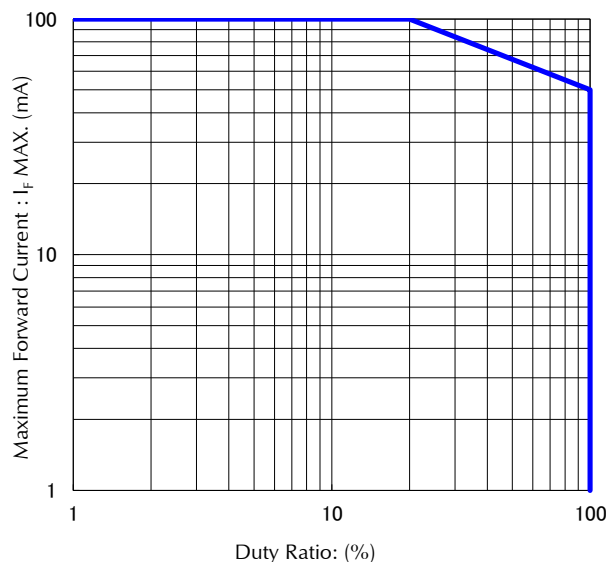
Duty Ratio vs. Max. Forward Current
