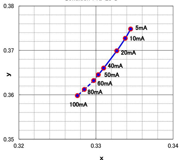
Chromaticity coordinates vs. Forward Current
