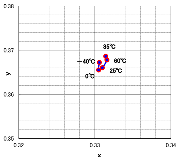
Chromaticity coordinates vs. Ambient Temp.
