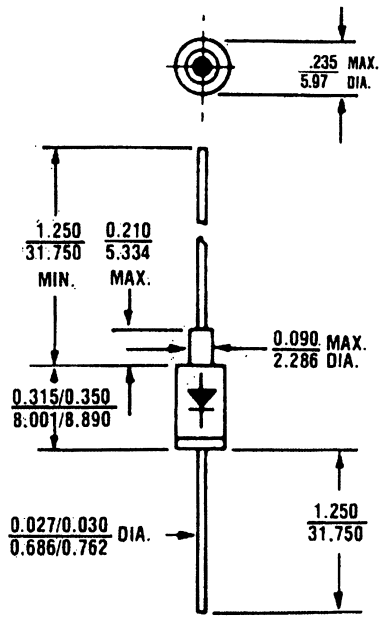
All dimensions in \frac{\text{INCH}}{\text{m.m.}} DO-13 (DO-202AA)
