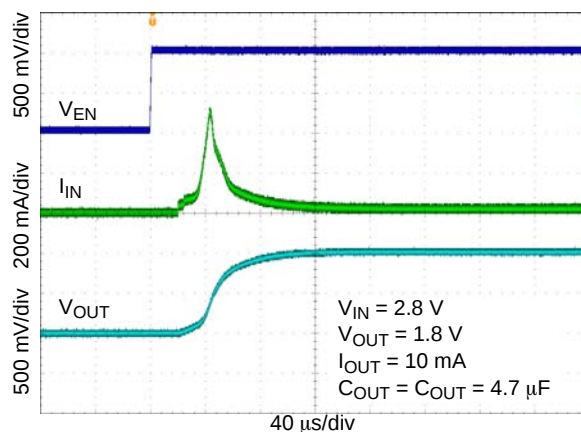
Figure 27. Enable Turn-on Response – V_{OUT} = 1.8 V , C_{OUT} = 4.7 \mu F
