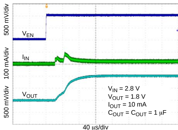
Figure 26. Enable Turn-on Response – V_{OUT} = 1.8 V , C_{OUT} = 1 \mu F
