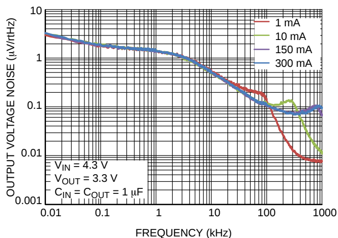
Figure 25. Output Voltage Noise Spectral Density for V_{OUT} = 3.3 V , C_{OUT} = 1 \mu F
