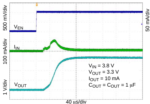
Figure 28. Enable Turn-on Response – V_{OUT} = 3.3 V , C_{OUT} = 1 \mu F
