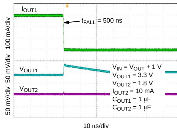
Figure 39. Load Transient Response – 1.8 V – Falling Edge, I_{OUT1} = 300 mA to 1 mA
