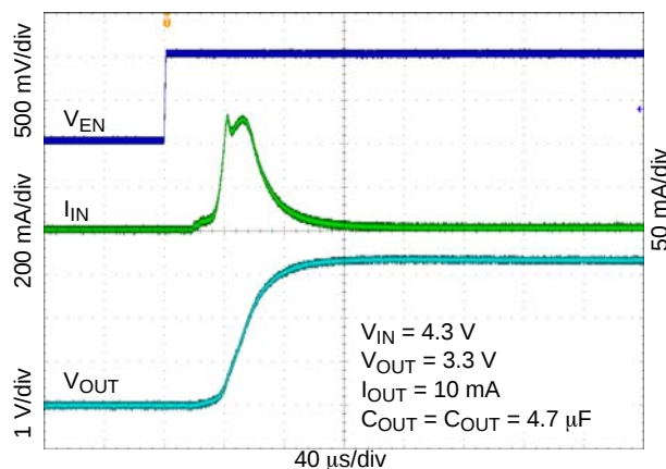
Figure 29. Enable Turn-on Response – V_{OUT} = 3.3 V , C_{OUT} = 4.7 \mu F
