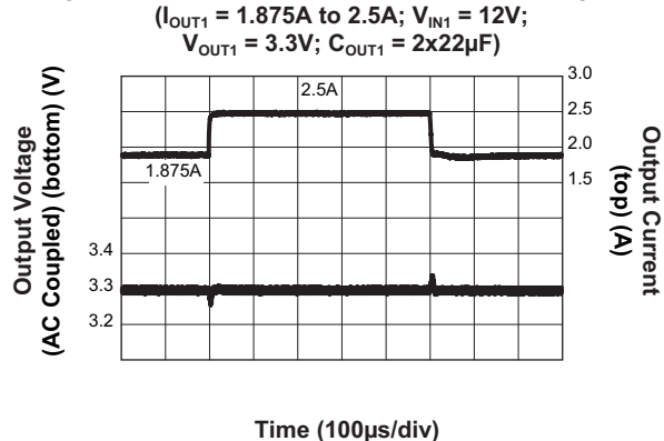
Step-Down Converter Load Transient Response ( I_{OUT1} = 1.875A to 2.5A ; V_{IN1} = 12V ; V_{OUT1} = 3.3V ; C_{OUT1} = 2 \times 22\mu F )
