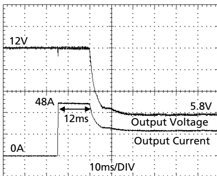
High Overload Current (typ. 48A for 12ms) enables easy fuse tripping
