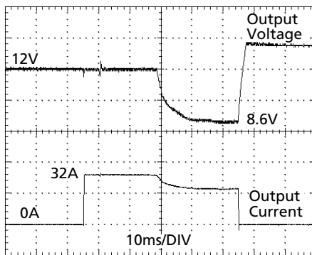
32A Peak load (resistive) for 50ms Output voltage dips from 12V to 8.6V.
