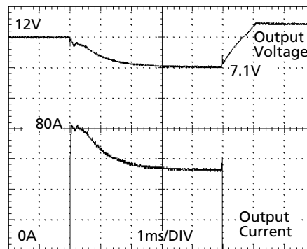
80A Peak load (resistive) for 5ms Output voltage dips from 12V to 7.1V.
