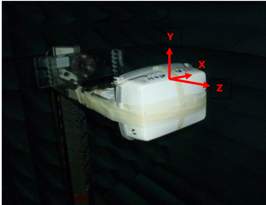
In ZRM 500 Housing
