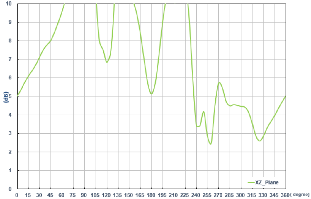
XZ Plane (phi=0° , Theta= -180~180° ), 0 degree face Zenith
