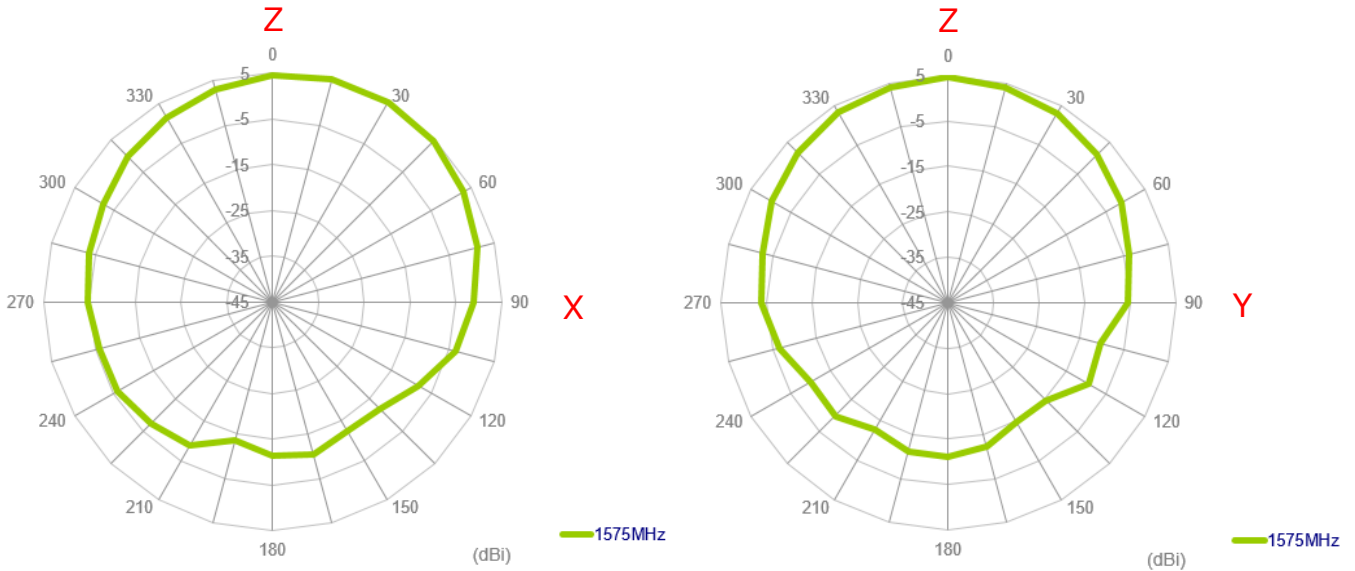
XZ Plane ( \phi=0^\circ , \theta ) YZ Plane ( \phi=90^\circ , \theta=0\sim 360^\circ )
