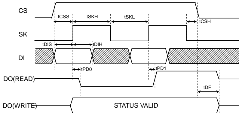
Figure 1. Sync data input / output timing
