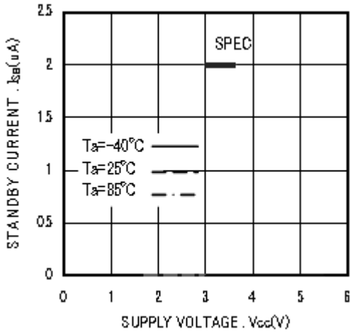
Figure 10. Consumption current at standby action Ibb
