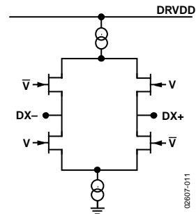
Figure 11. Data Outputs (LVDS Mode)
