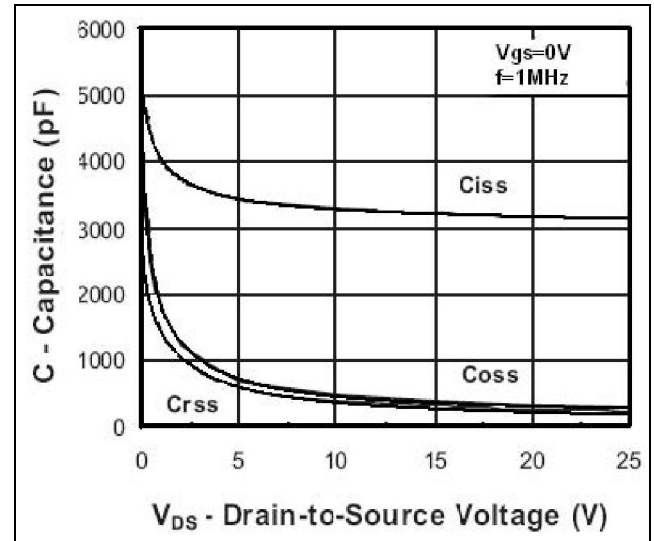
Capacitance
