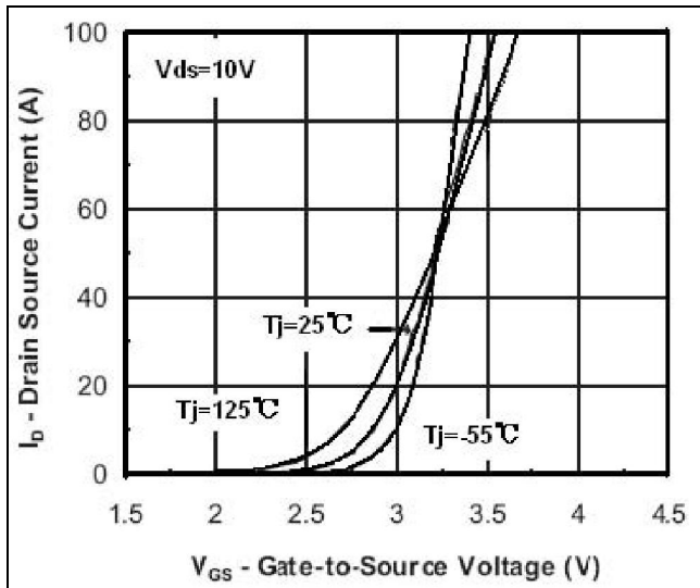
Transfer Characteristic
