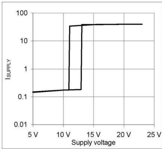
Fig. 1 - Supply Current
