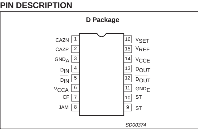
Figure 1. Pin Configuration
