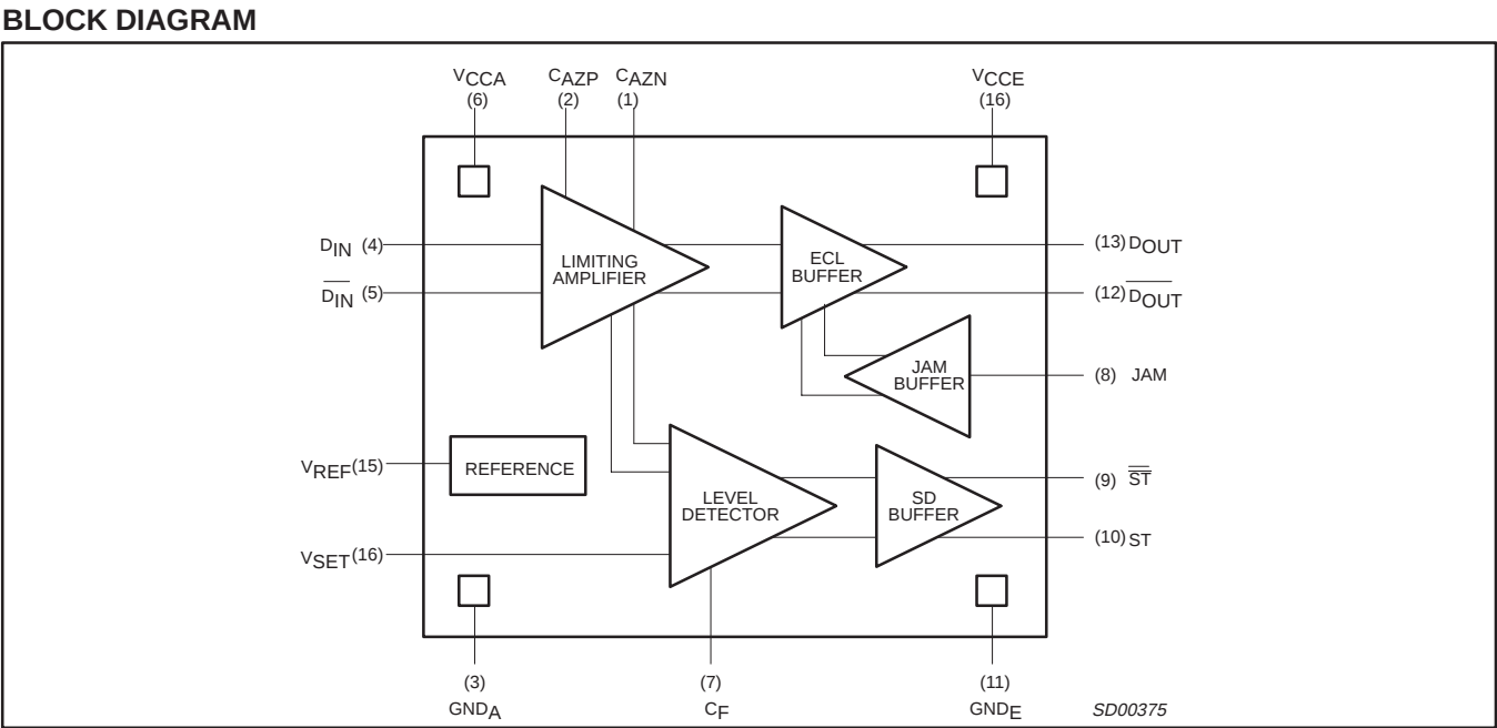
Figure 2. Block Diagram
