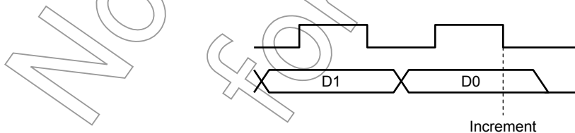
Figure 11 Increment Timing Diagram
