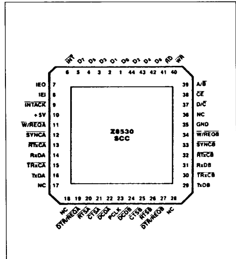
Figure 4 : Chip Carrier Pin Connection.
