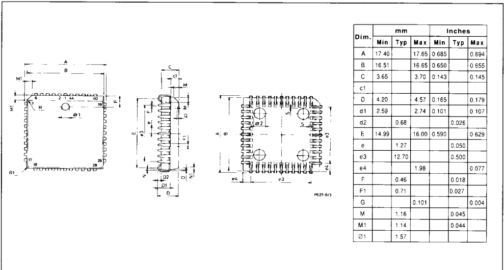
Figure 83 : Z8530 44-Lead Plastic Leaded Chip Carrier.
