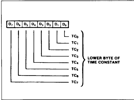
Figure 55 : Write Register 12.
