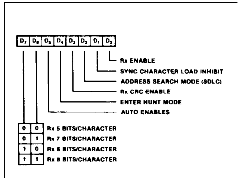
Figure 62 : Write Register 3.
