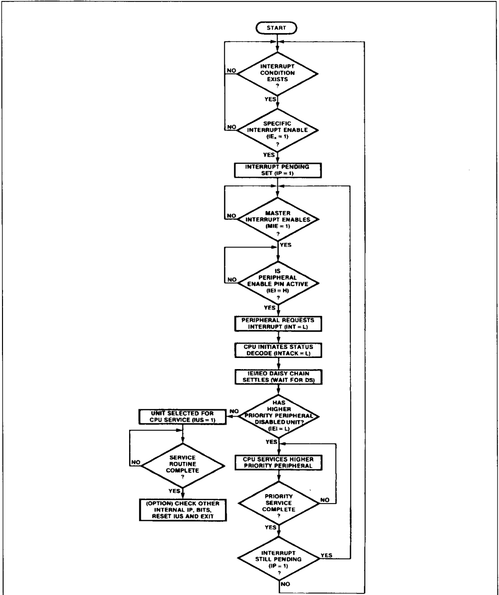
Figure 17 : Interrupt Flowchart.
