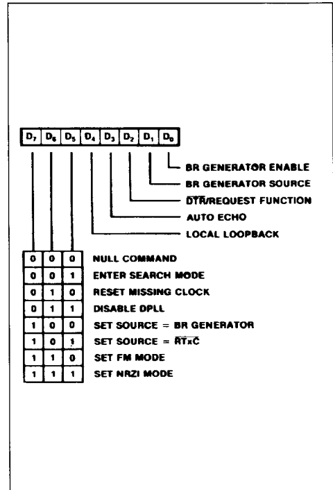
Figure 57 : Write Register 14.
