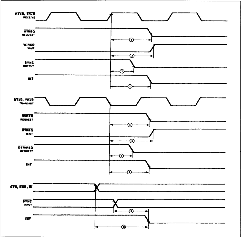
Figure 80 : System Timing.
