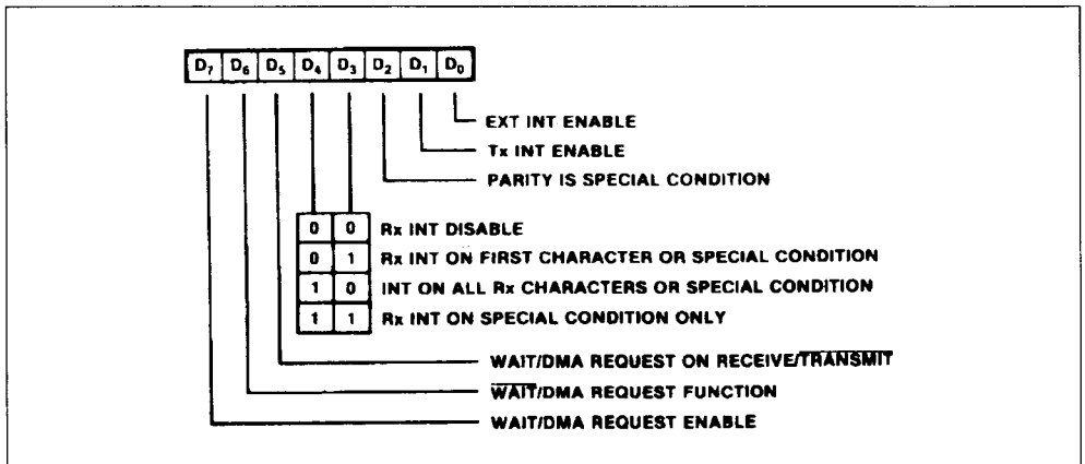
Figure 44 : Write Register 1.
