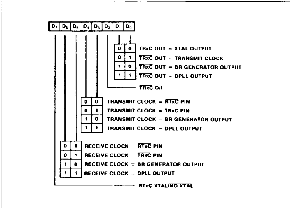
Figure 54 : Write Register 11.
