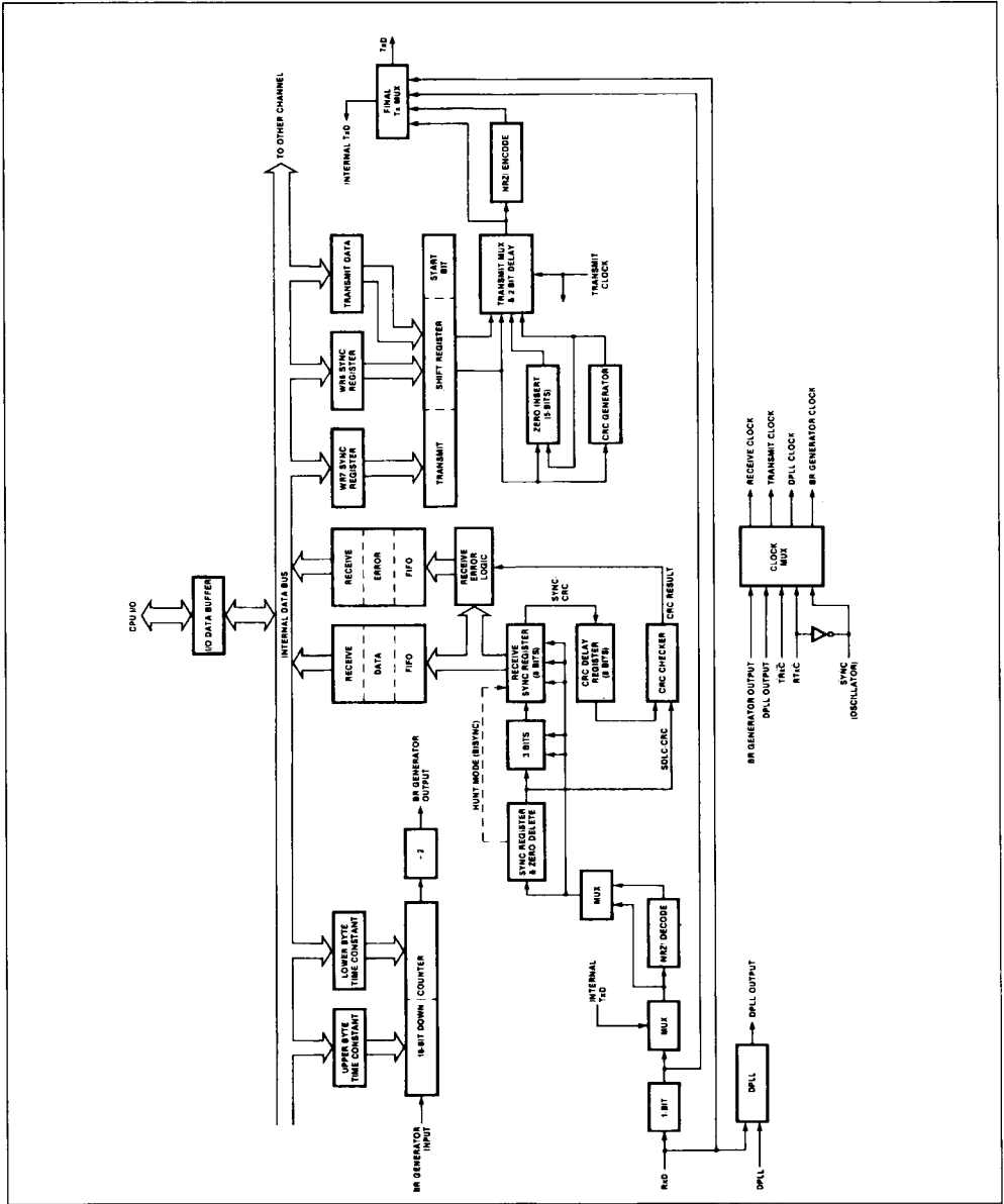
Figure 5 : Data Paths.
