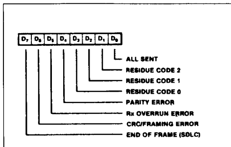
Figure 60 : Read Register 1.
