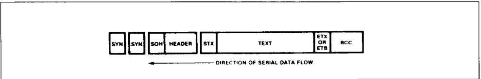
Figure 10 : External Sync Format.
