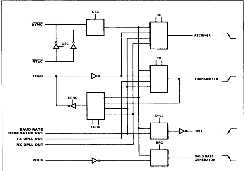
Figure 32 : Clock Multiplexer.
