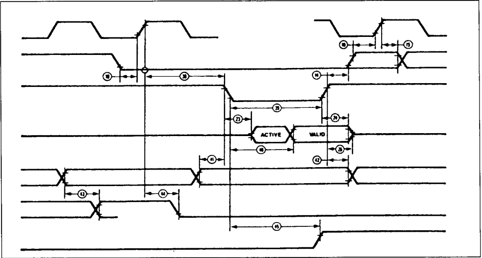
Figure 77 : Reset Timing.
