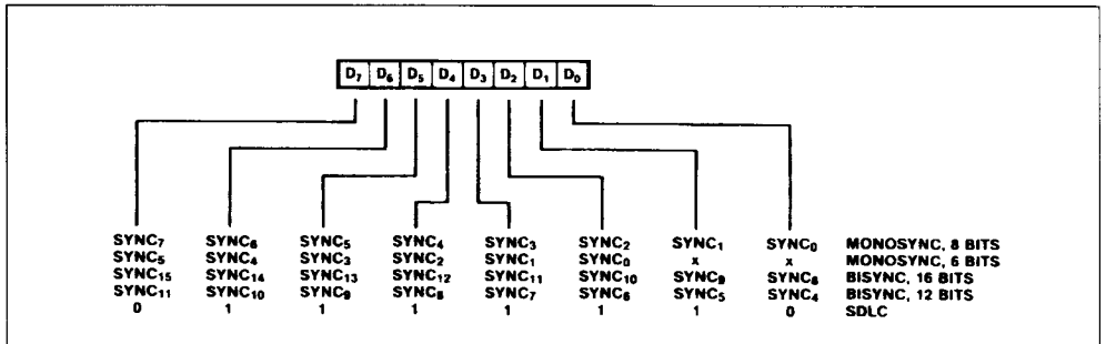
Figure 49 : Write Register 6.
