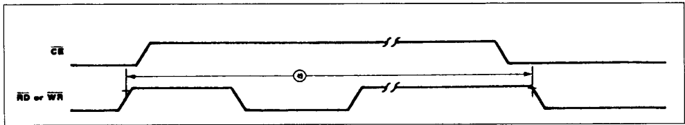
Figure 78 : Cycle Timing.
