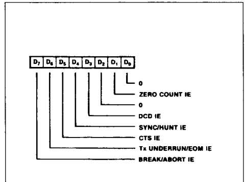
Figure 66 : Write Register 15.
