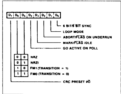
Figure 52 : Write Register 10.
