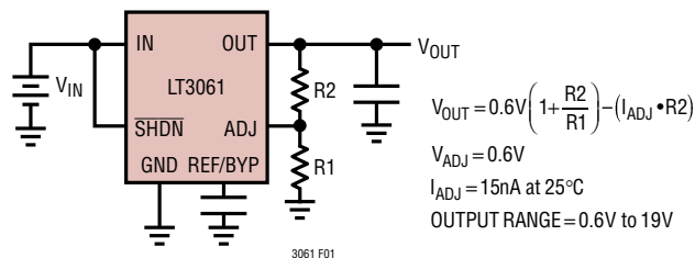
Figure 1. Adjustable Operation
