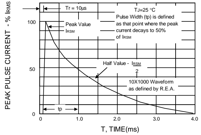
FIG.2 - PULSE WAVEFORM
