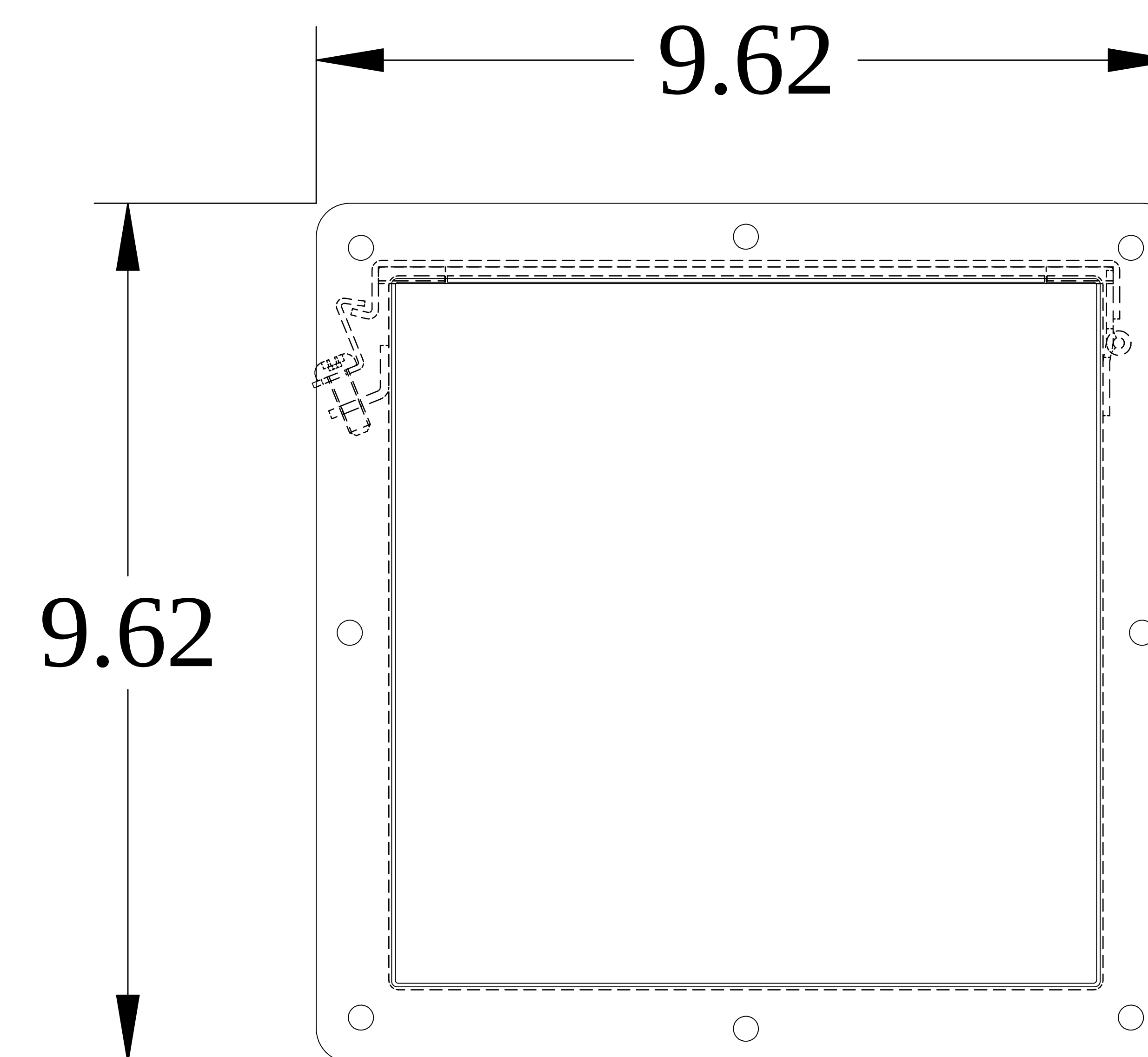
END VIEW
