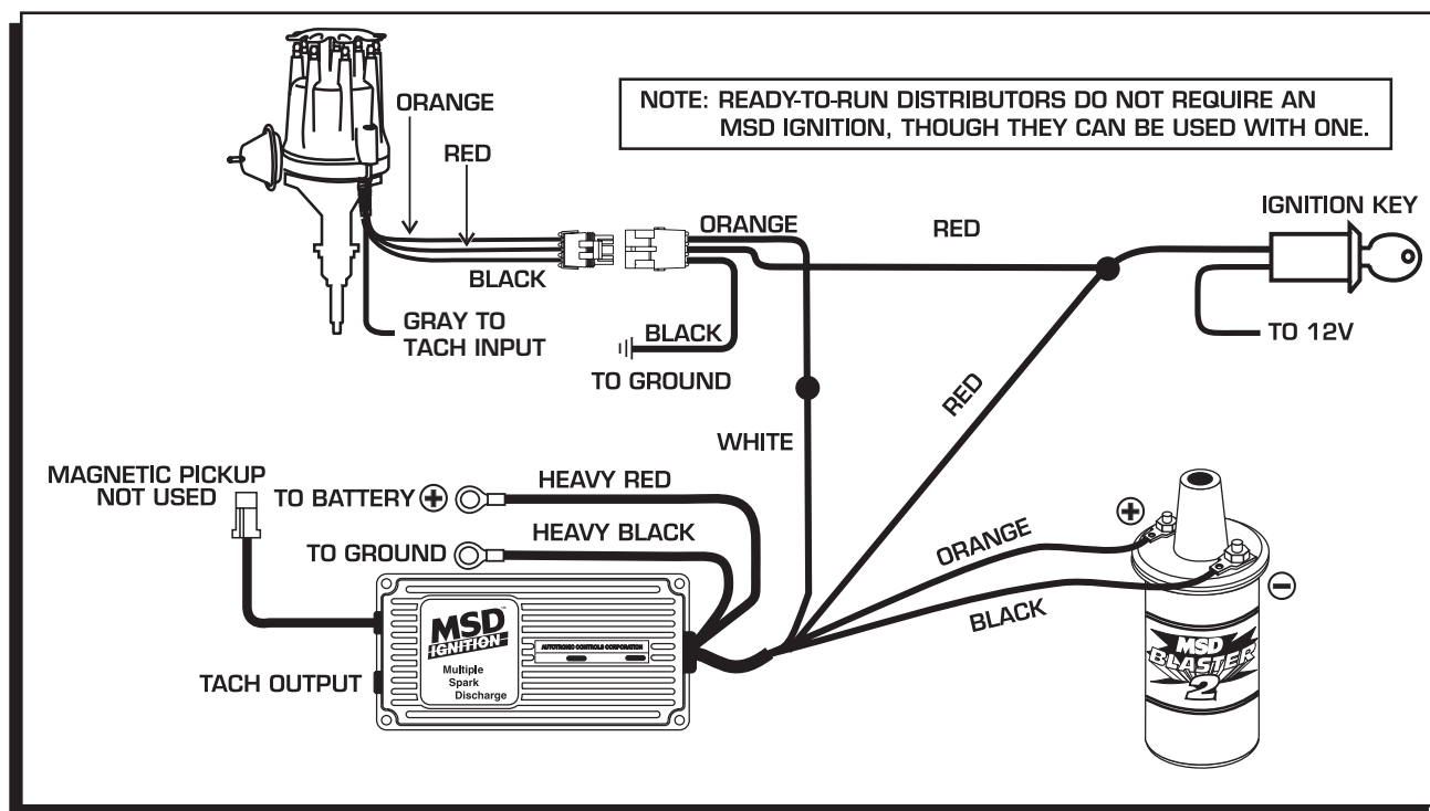
Figure 15 Wiring to an MSD Ignition Control.
