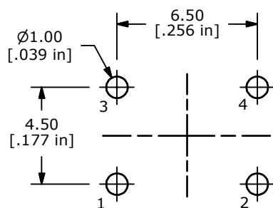
P.C.B. MOUNTING
