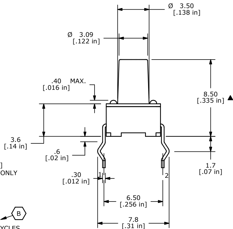
P.C.B. MOUNTING
