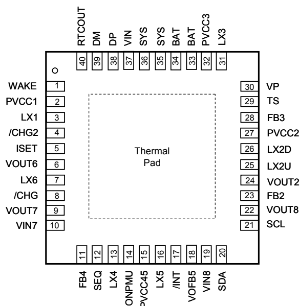
G2206 TQFN5X5-40
