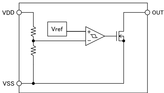
N-ch Output
