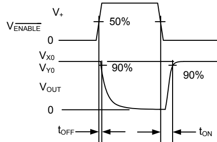
Test Circuit 2. Enable Switching Times ( t_{ON} , t_{OFF} )
