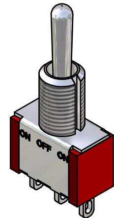
ISOMETRIC
