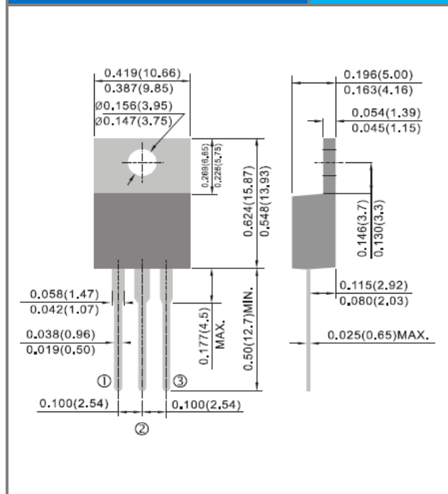
TO-220AB Dimension
