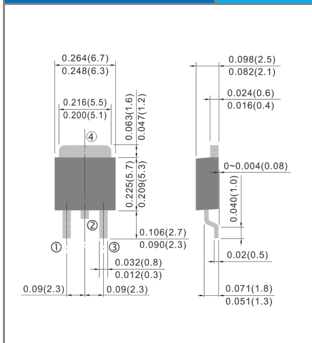
TO-252 Dimension
