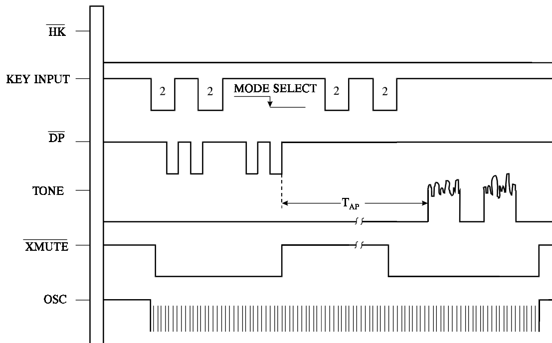
Figure 4. Normal Pulse to Tone mixed dialing via slide switch
