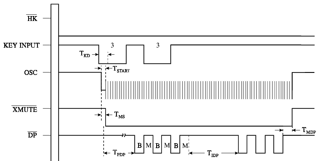
Figure 2. Pulse Mode
