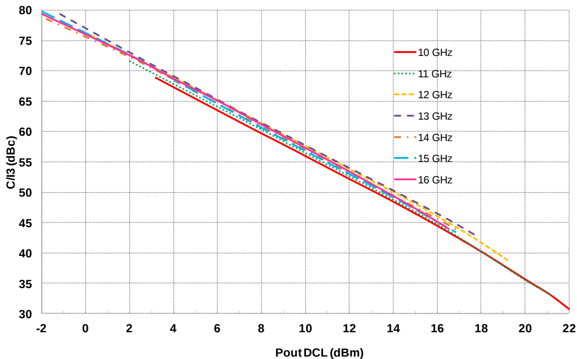
C/I3 versus Pout DCL & frequency
