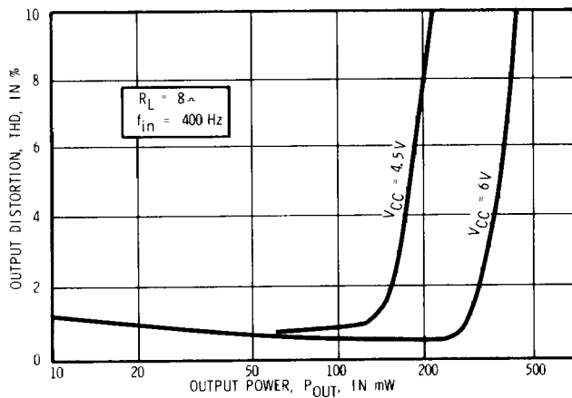
TOTAL HARMONIC DISTORTION WITH 8 \Omega LOAD
