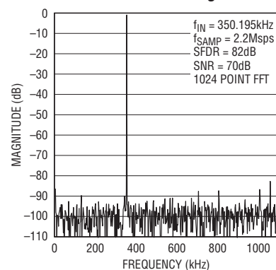
350kHz FFT Driving ADC
