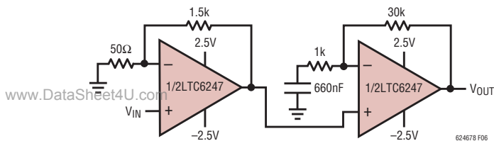
Figure 6. 60dB 5.5MHz Gain Block
