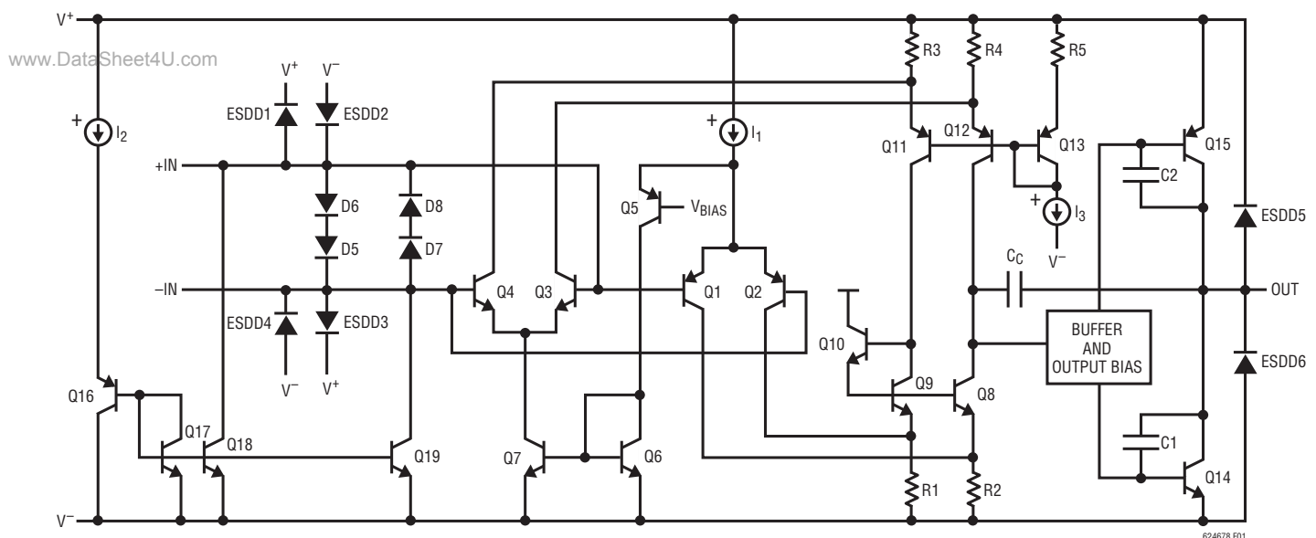
Figure 1. LTC6246/LTC6247/LTC6248 Simplified Schematic Diagram
