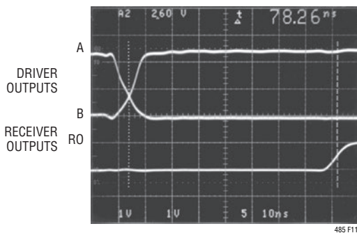
Figure 11. Receiver t_{PHL}
