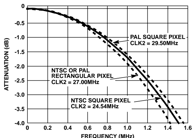
FIGURE 9B. PASS BAND
