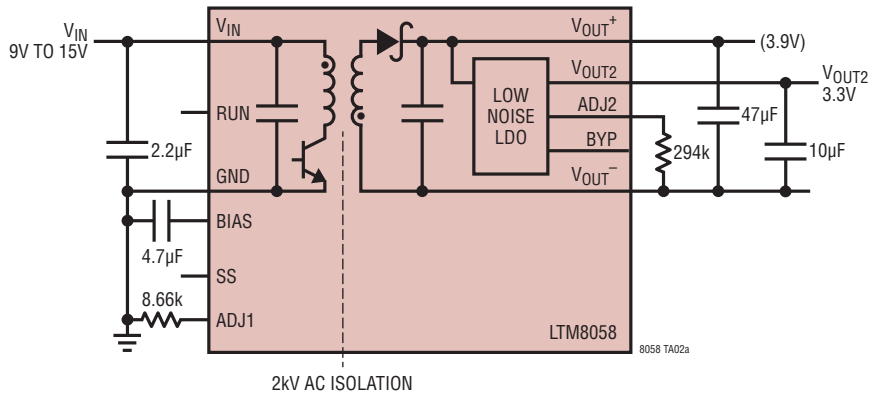
3.3V Flyback Converter
