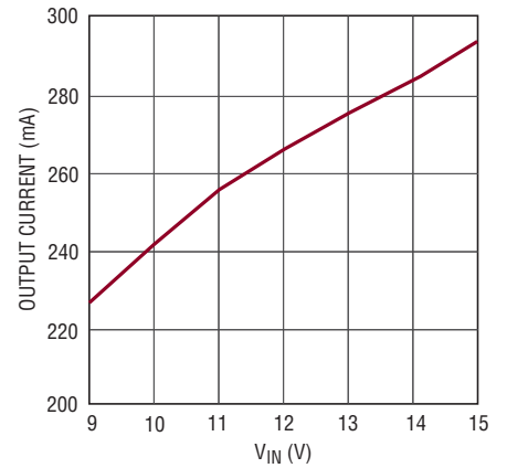
V OUT2 Maximum Output Current vs V IN
