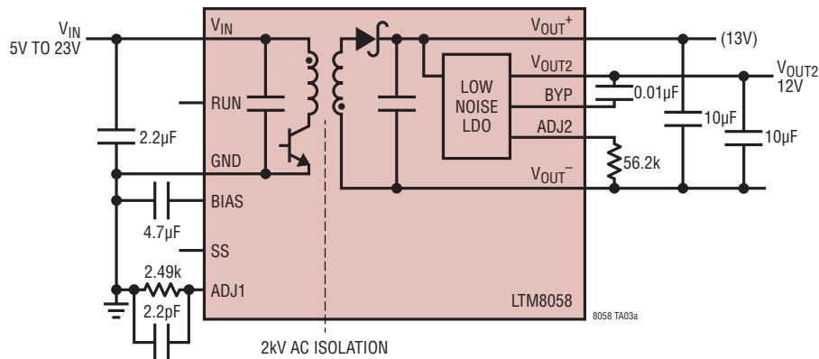
12V Flyback Converter with Low Noise Bypass
