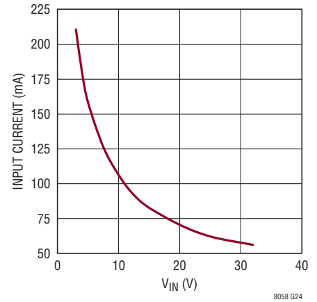
Input Current vs V_{IN} , V_{OUT2} Shorted
