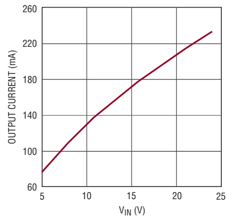
V OUT2 Maximum Output Current vs V IN
