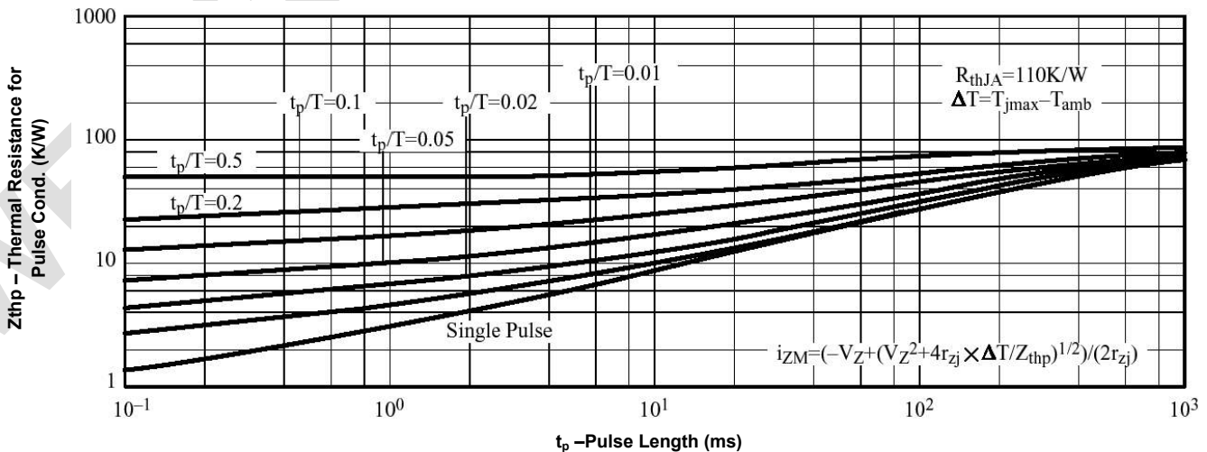
Figure5. Thermal Response
