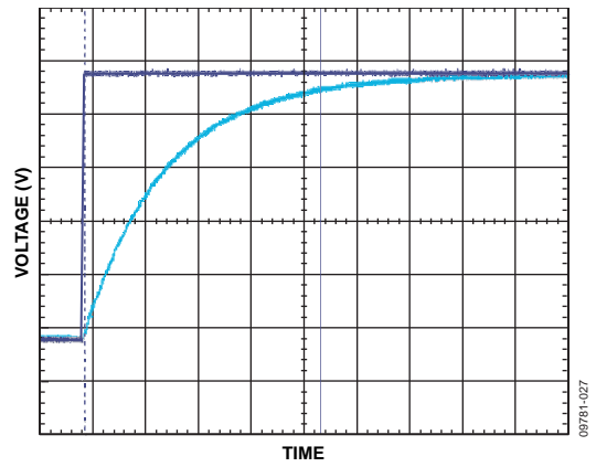
Figure 38. Turn-On Time; C x , C y = 0.1 μF, Time Scale = 2 ms/DIV
