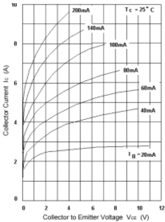
Fig.3 Static Characteristic
