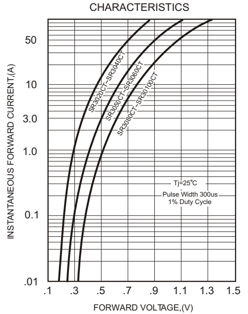
FIG.2-TYPICAL FORWARD CHARACTERISTICS
