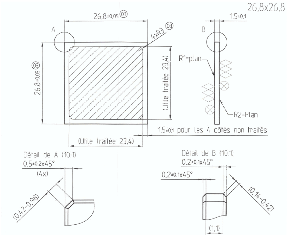
Figure 4. Glass Lid Dimensions
