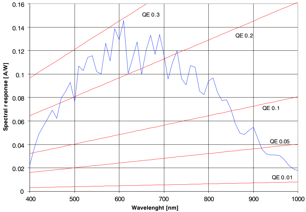
Figure 10. Spectral Response
