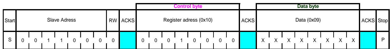
Figure 16: I 2 C write
