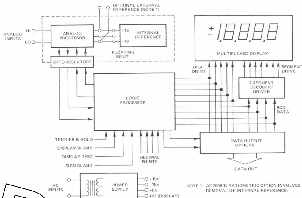
Figure 1. AD2008 Block Diagram
