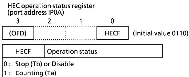
Figure 3-6. HEC operation status register
