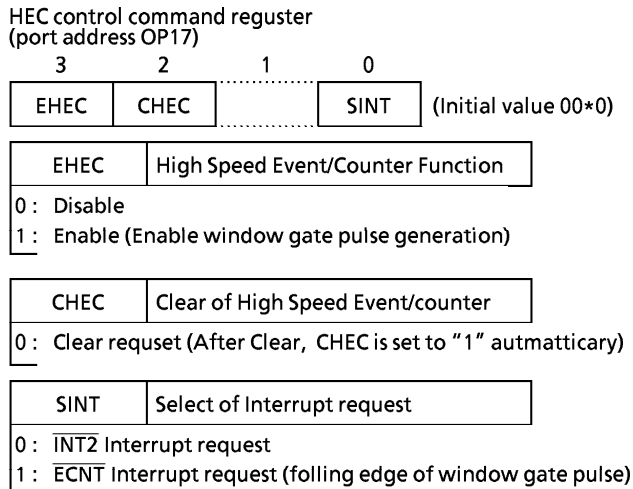
Figure 3-4. HEC Control Command Register
