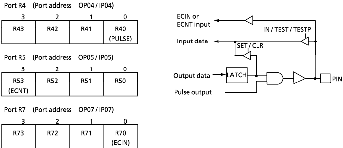
Figure 3-2. Port R4, R5, R7
