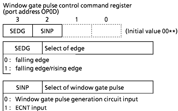
Figure 3-5. Window gate pulse control command register
