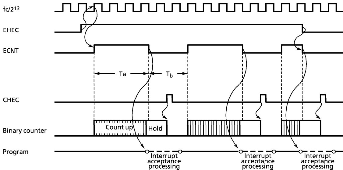
Figure 3-7. HEC Operation Timing
