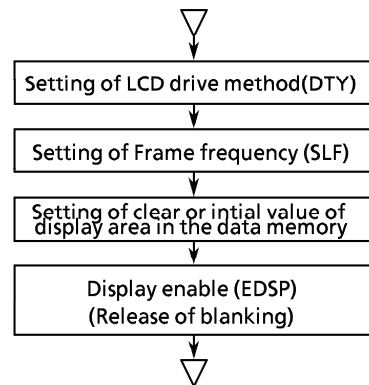
Figure 3-15. Initial setting of LCD driver
