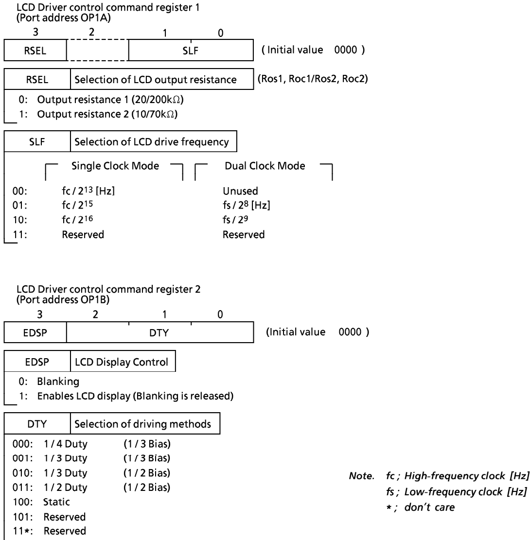
Figure 3-12. LCD Driver control Command Register
