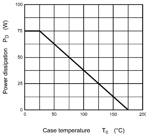
Fig. 8.11 P_D - T_c (Guaranteed Maximum)
