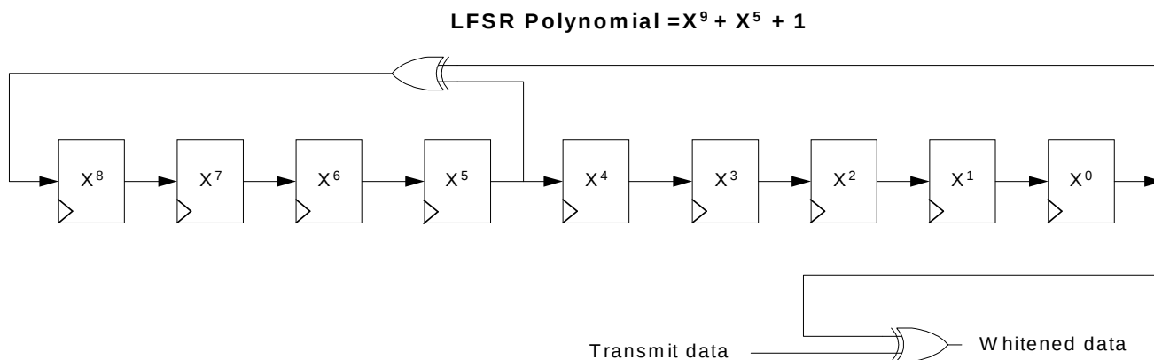
Figure 47: Data Whitening
