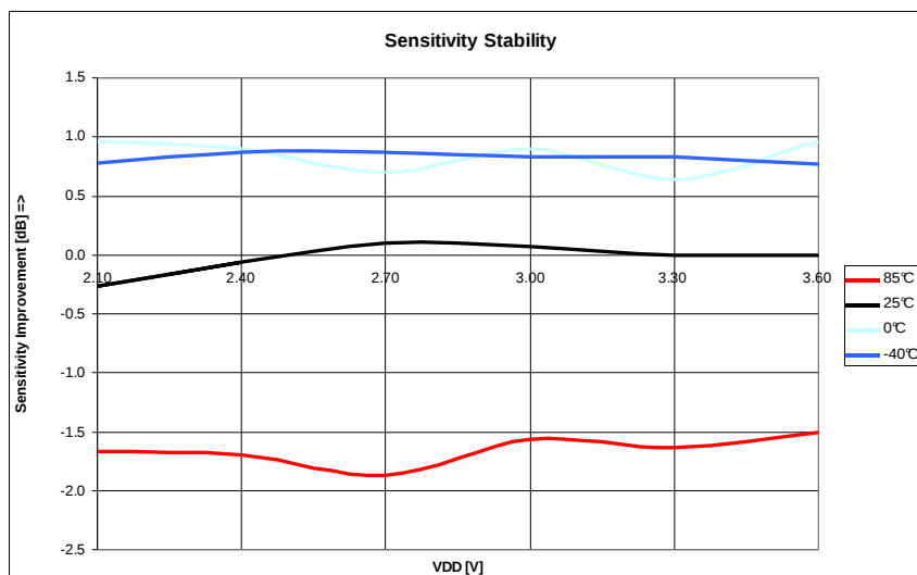
Figure 67: Sensitivity Stability
