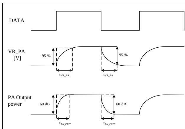
Figure 10: PA Control
