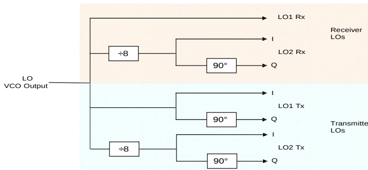
Figure 6: LO Generator
