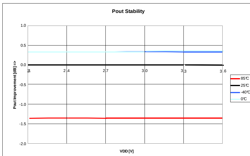
Figure 76: Pout Stability
