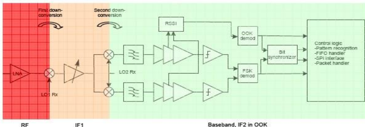
Figure 14: Receiver Architecture
