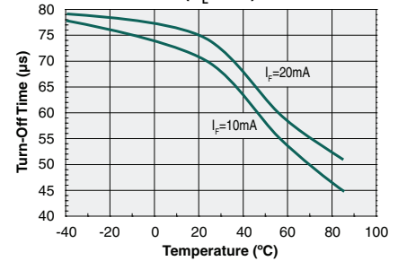
Typical Turn-Off Time vs. Temperature (V L =10V)
