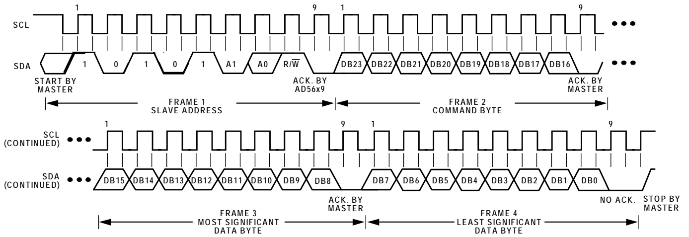
Figure 74. I 2 C Read Operation
