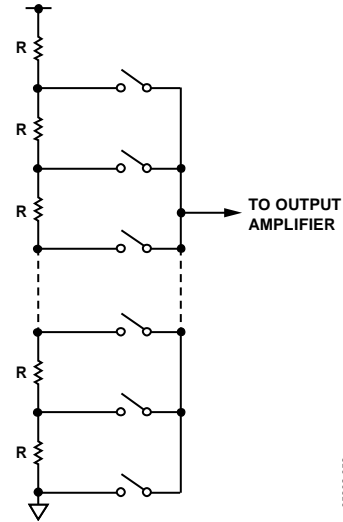
Figure 72. Resistor String
