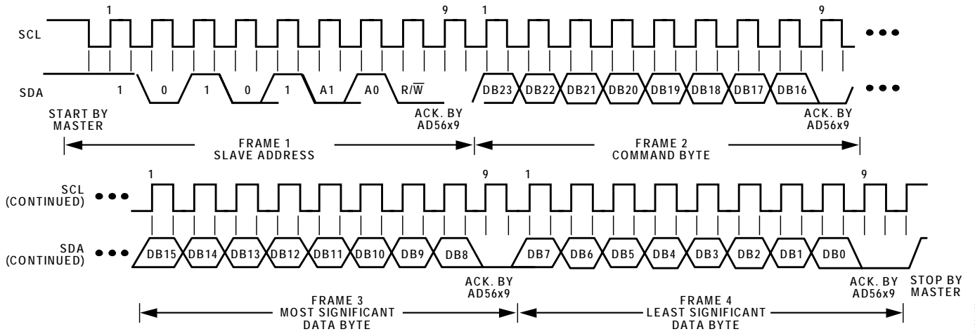
Figure 73. I 2 C Write Operation
