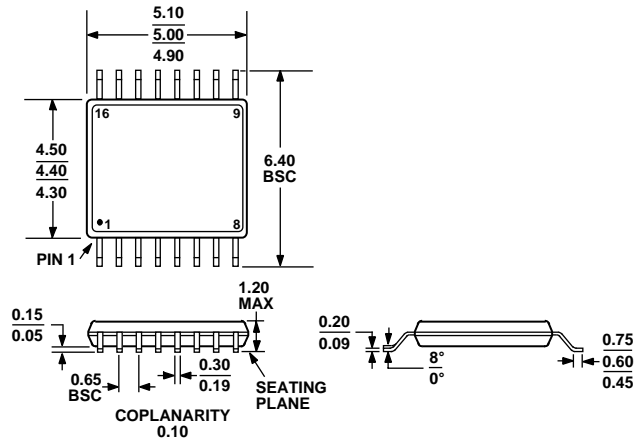
Figure 79. 16-Lead Thin Shrink Small Outline Package [TSSOP] (RU-16)
