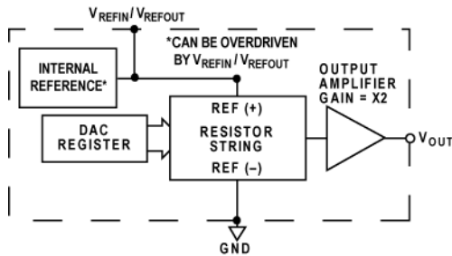
Figure 70 DAC Architecture for internal reference configuration
