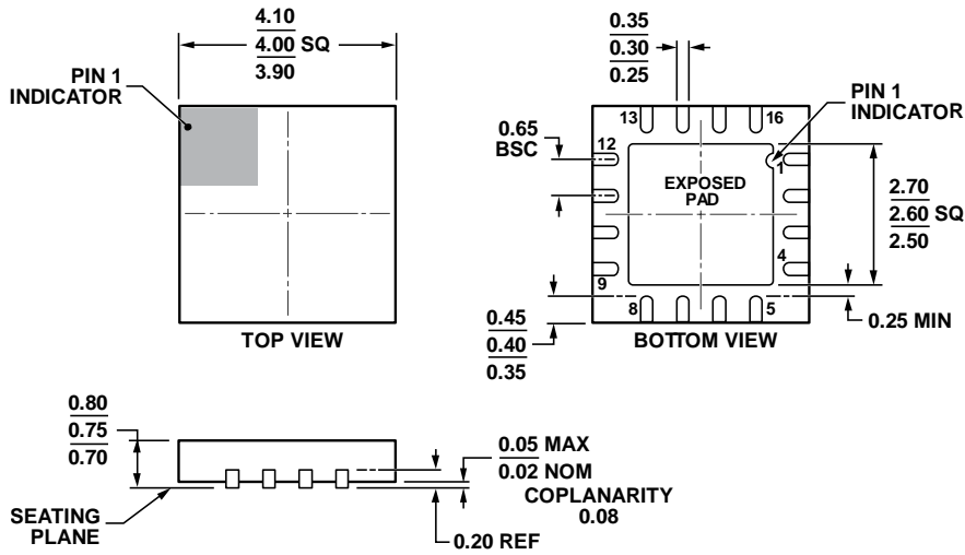
Figure 78. 16-Lead Lead Frame Chip Scale Package [LFCS] (CP-16-17)
