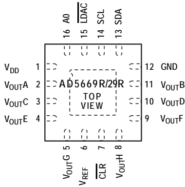
Figure 2. 16-Lead LFCSP (CP-16-17)
