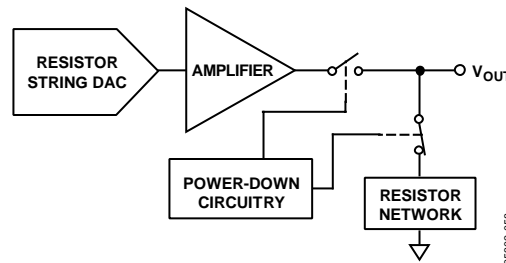
Figure 77. Output Stage During Power-Down
