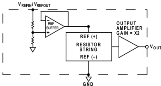
Figure 71. DAC Architecture for external reference configuration
